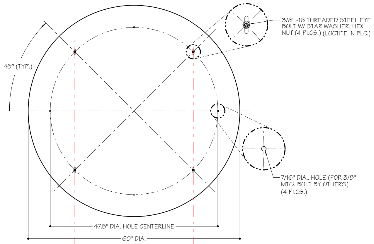
MTG. PLATE TOP VIEW
